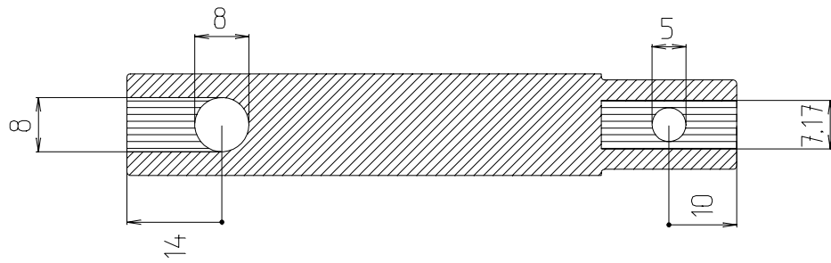
PART A - Side view
