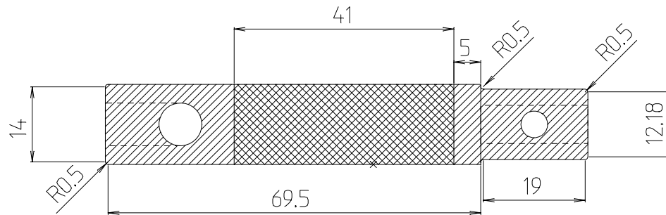
PART A - Side view
