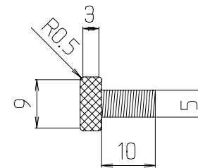
PART B - Side view
