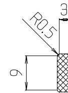
PART C - Side view
